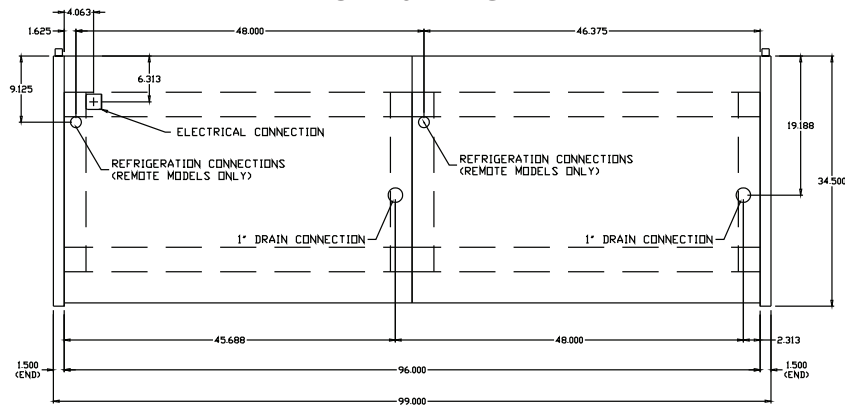
8' Plan View
