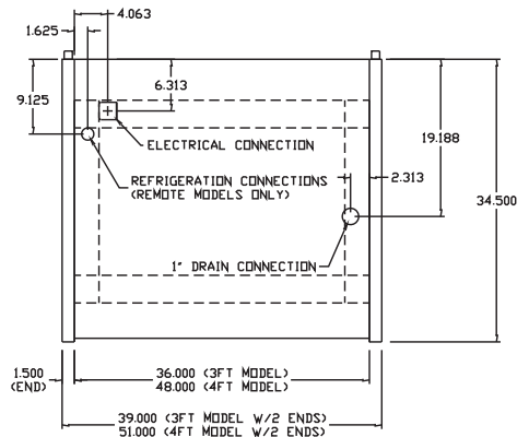
3' & 4' Plan Views
